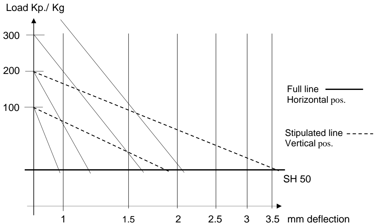
Load / deflection chart
