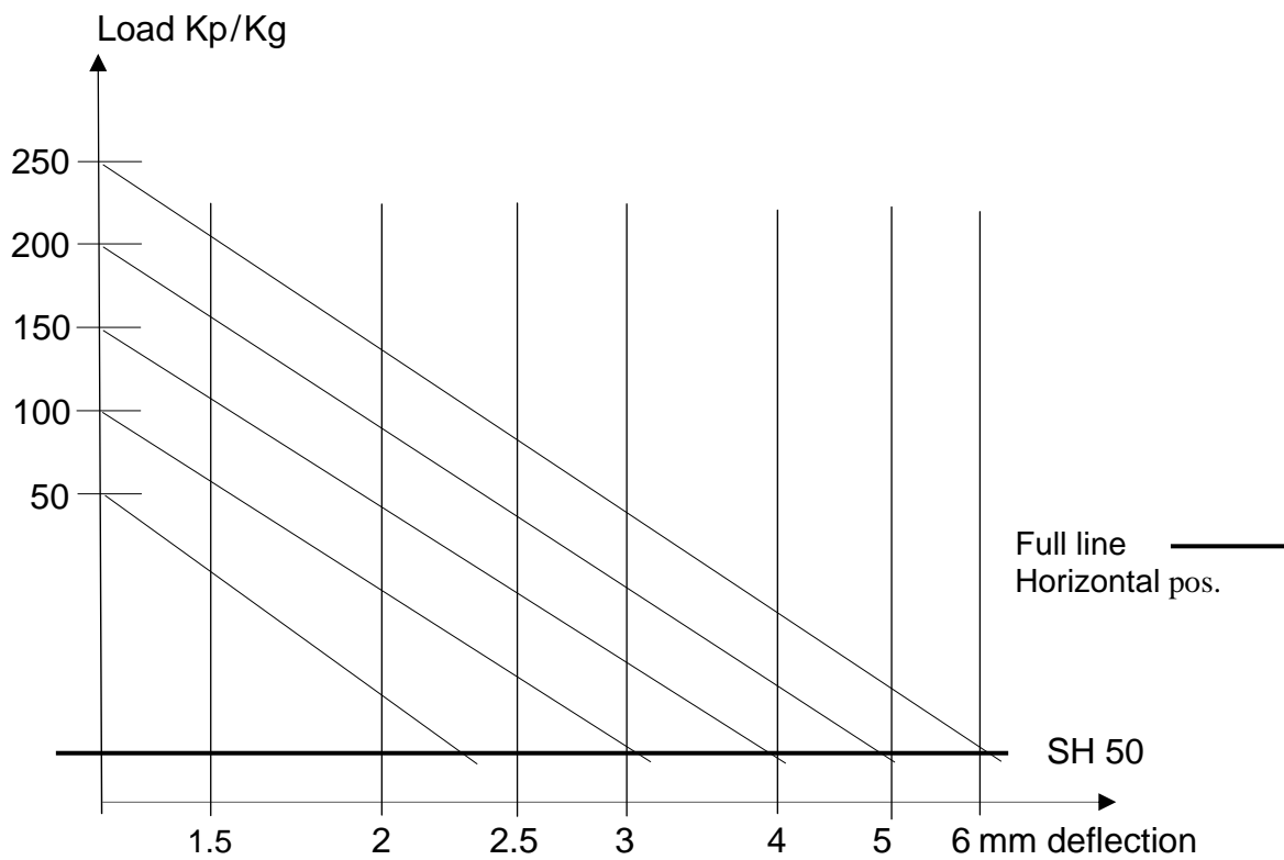
Load / deflection chart
